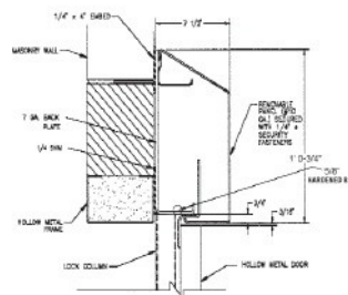
COVER BOX SECTION 7-1/2" deep x 1'-2/4" tall cover box field welded 1" on 8" top and bottom.
